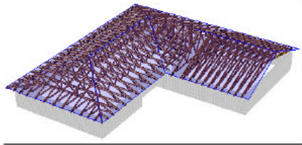
Roof surface transparency
