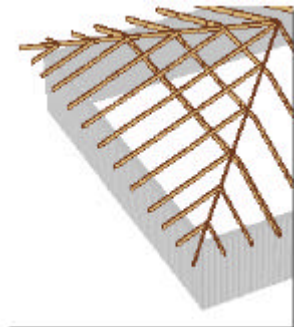
Level rafter
